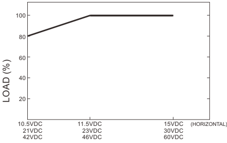
Battery Input Voltage (V) Figure 7.3 Input Derating Curve
