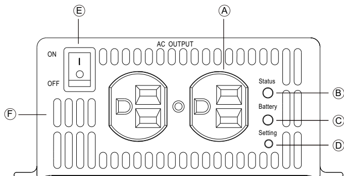
Figure 3.1 Front Panel(Type A)
