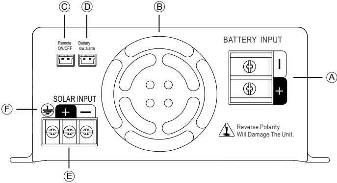
Figure 3.2 Rear Panel
